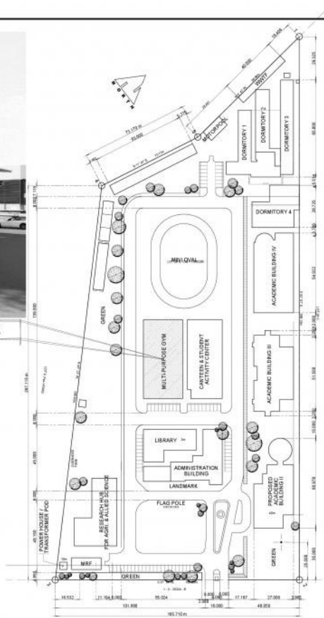
03 SITE DEVELOPMENT PLAN A-01 SCALE
